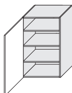
W4/60/1 600/960/325
