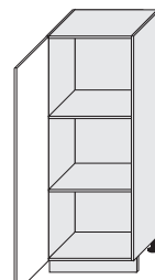
D5D/60/154 600/1540/565
