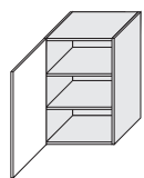
W2/50 500/720/325
