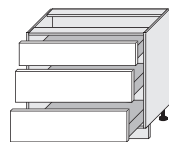
D3A/90 D3M/90 D3R/90 900/820/500
